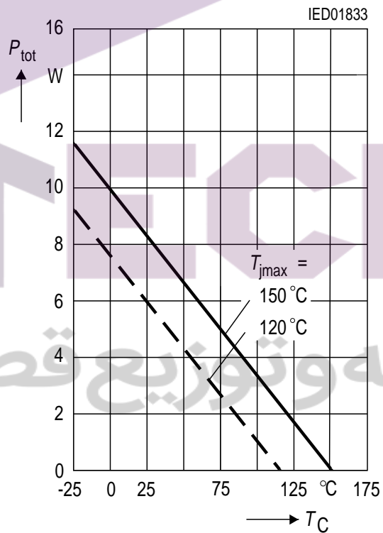
Permissible Power Dissipation P_{tot} versus Case Temp. T_C (measured at pin 5)
