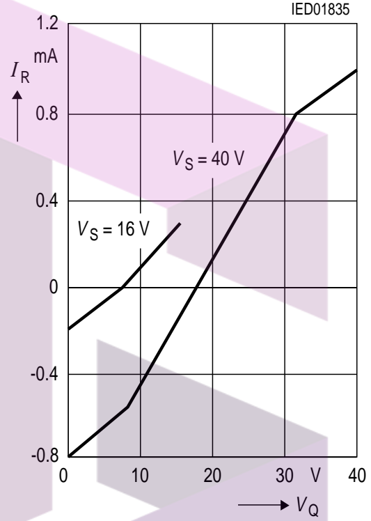
Output Leakage Current
